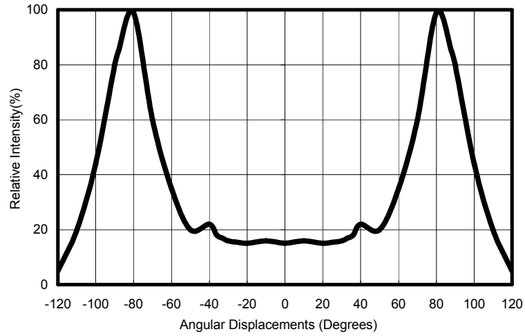
<Figure 9.Side emitting at T_j=25^{\circ}\text{C} for all color.>
