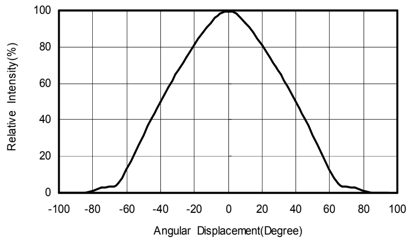
<Figure 11.Focusing at T_j=25^{\circ}\text{C} for cool white.>
