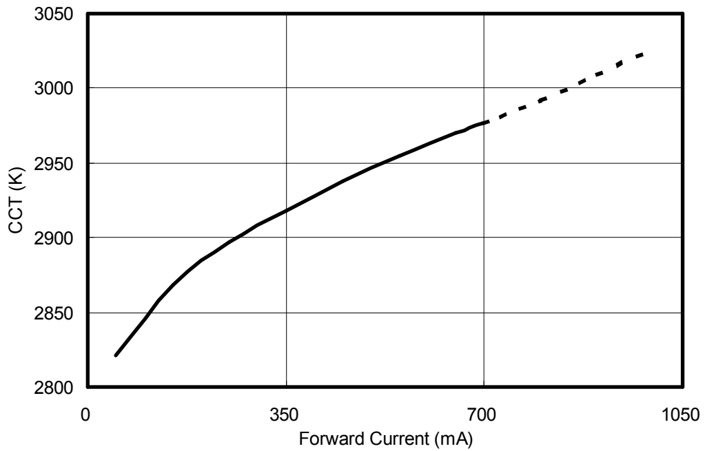
< Figure 20. Forward current & CCT at T_j=25^\circ\text{C} for Edixeon ® series warm white >
