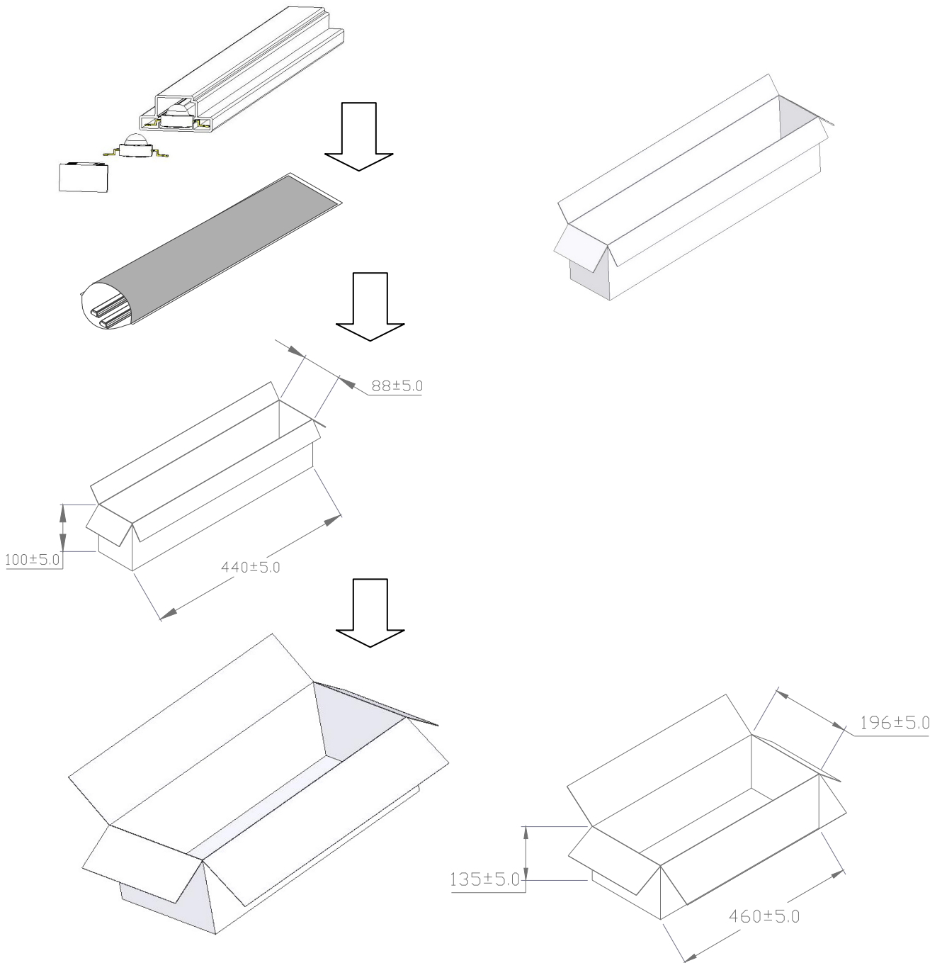
<Figure 30. Package steps and dimensions >
