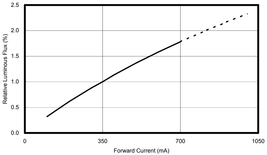
< Figure 17. Forward current & relative luminous at T_J=25^\circ\text{C} for 3W Edixeon ® series >
