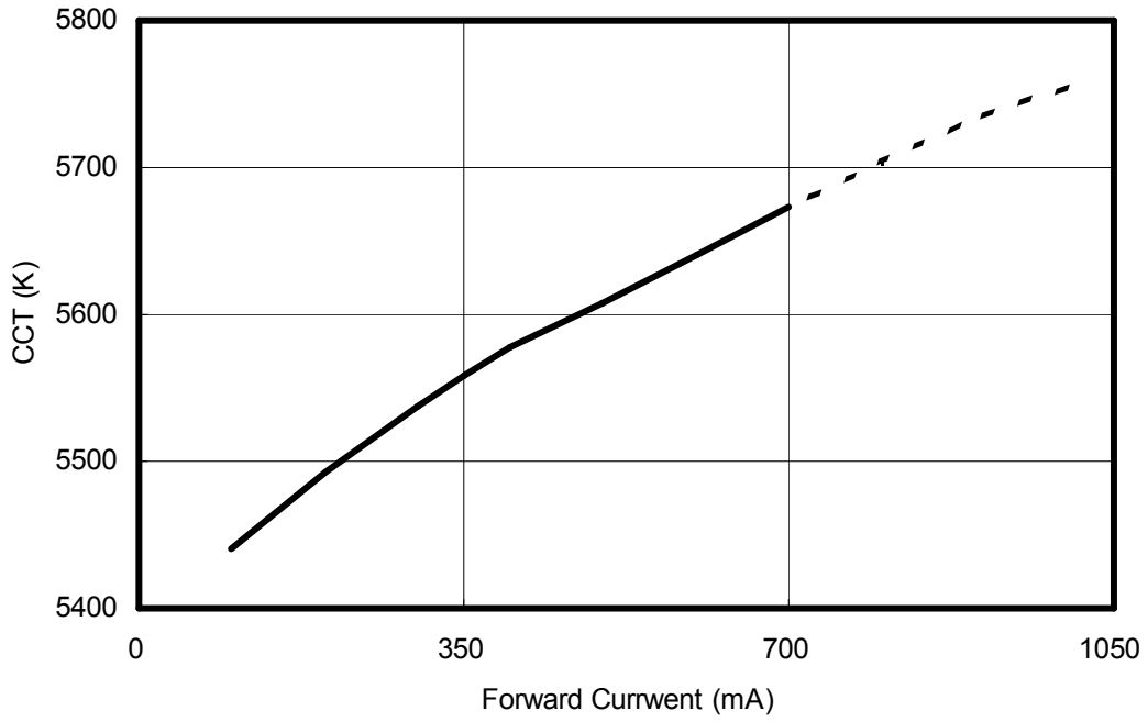
< Figure 18. Forward current & CCT at T_J = 25^\circ\text{C} for Edixeon ® series cool white >
