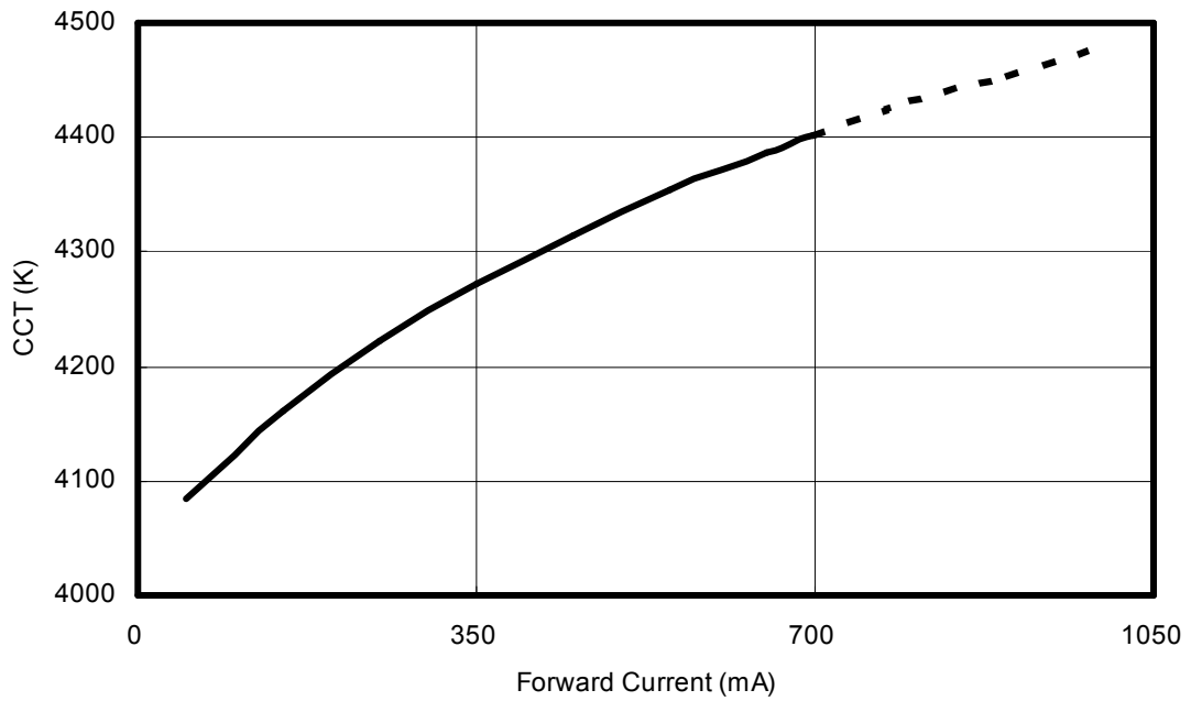
< Figure 19. Forward current & CCT at T_J = 25^\circ\text{C} for Edixeon ® series neutral white >
