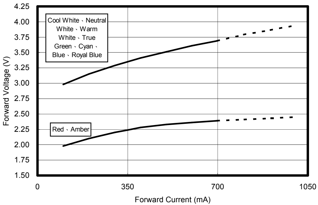
< Figure 15. Forward current & forward voltage for 3W Edixeon® series >
