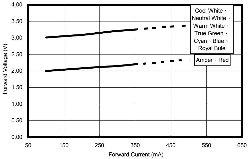
< Figure 14. Forward current & forward voltage for 1W Edixeon® series >
