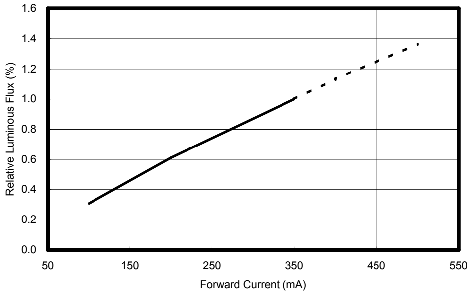
< Figure 16. Forward current & relative luminous at T_J=25^\circ\text{C} for 1W Edixeon ® series >
