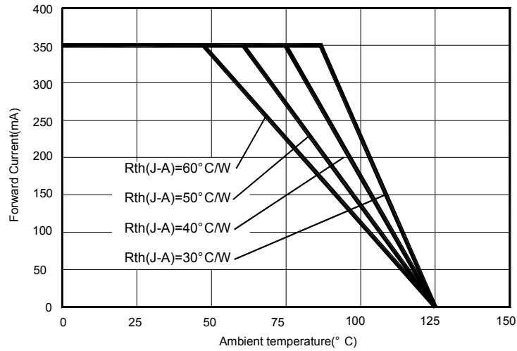
< Figure 12. Operating current & ambient temperature for 1W Edixeon ® series >
