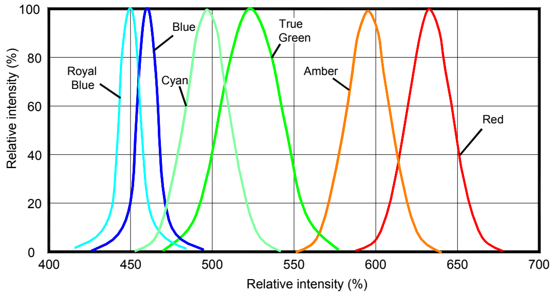
< Figure 5 Red, amber, true green, cyan, blue, dental blue, and royal blue color spectrum at T_j = 25^\circ\text{C} .for Edixeon ® series >
