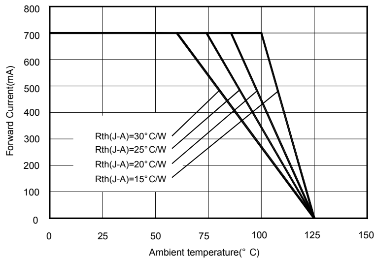
< Figure 13. Operating current & ambient temperature for 3W/5W Edixeon ® series >
