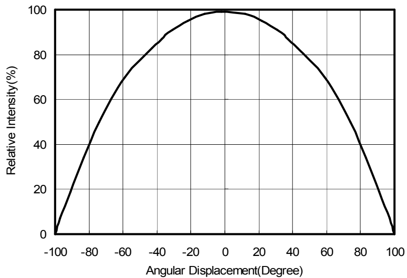
< Figure 8.Lambertain at T_J=25^{\circ}\text{C} for blue, dental blue, royal blue, cyan, and true green >
