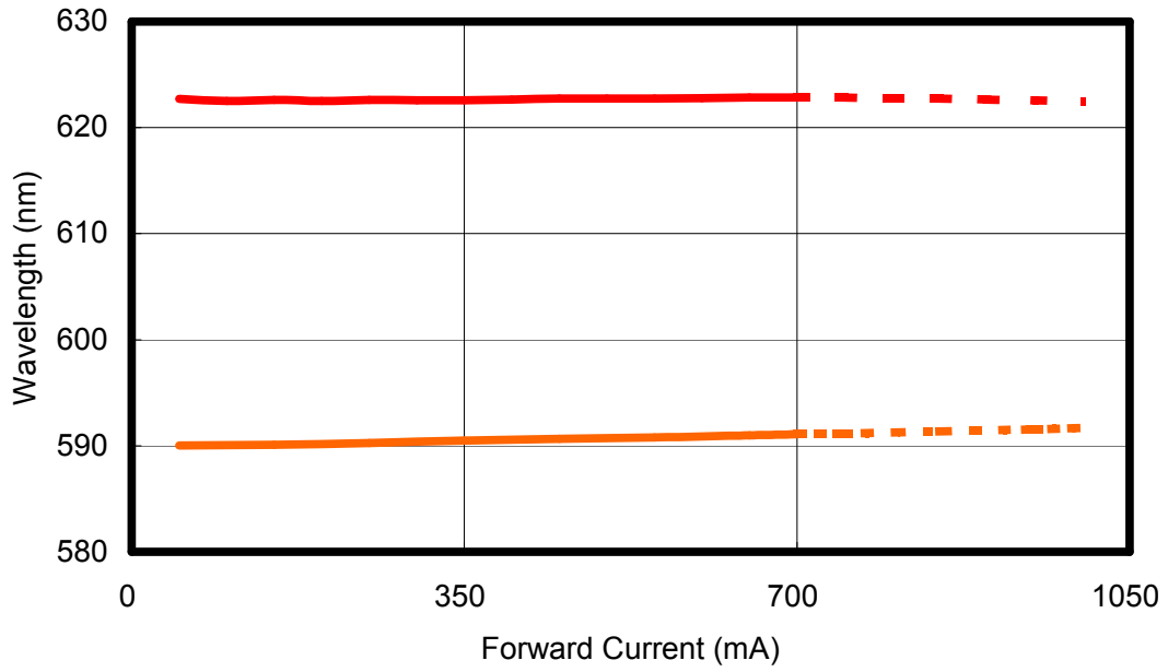
< Figure 22. Forward current & wavelength at T_J=25^{\circ}\text{C} for Edixeon ® series red and amber >
