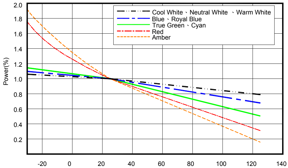
< Figure 23. Junction temperature & power rate for Edixeon ® series >
