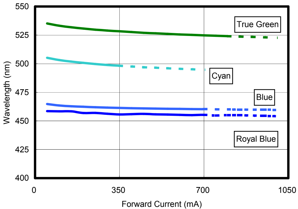
< Figure 21. Forward current & wavelength at T_j=25^\circ\text{C} for Edixeon ® series true green, blue, and royal blue >
